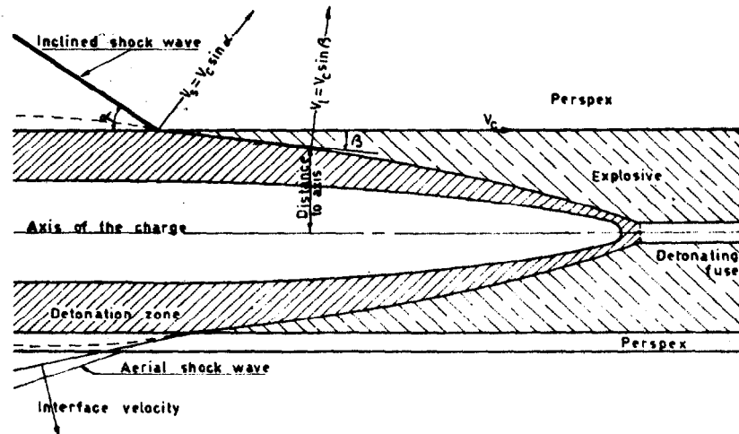
Fig 2 - Aspect of the detonation zone in explosive and the shock wave generated in surrounding medium
